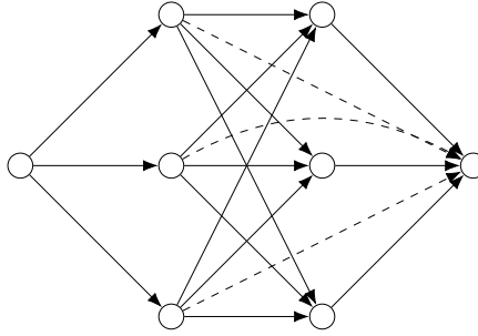
FIGURE 1. Example of a multi-stage DAG with homogeneous dependencies. Solid arrows denote dependencies between adjacent stages and dashed arrows denote dependencies between non-adjacent stages.
