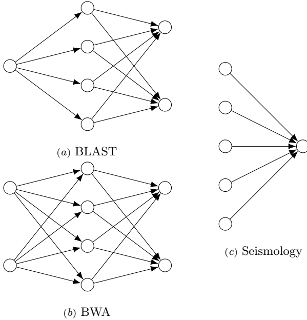
FIGURE 3. Graph structure examples
