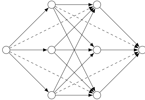
FIGURE 2. An approximately multi-stage DAG with homogeneous dependencies may not have the full set of all-to-all dependencies between the input task and some layer or between some layer and the output task, but these dependencies must have very small size.
